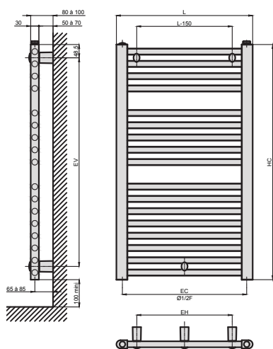
HYDRONIC VERSION
