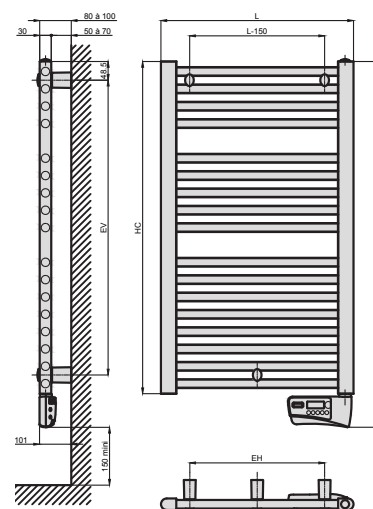
ELECTRIC VERSION
