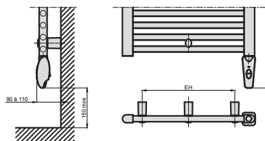
MIXED VERSION MID CONNECTION 50 mm
