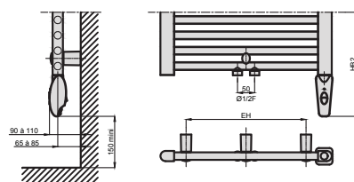
MIXED VERSION RF MID CONNECTION 50 mm
