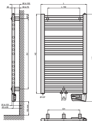
MIXED VERSION MID CONNECTION 50 mm
