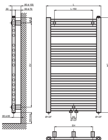
HYDRONIC VERSION MID CONNECTION 50 mm
